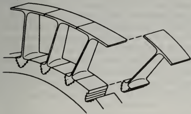
FIGURE 1-56. Shrouded turbine blades.
